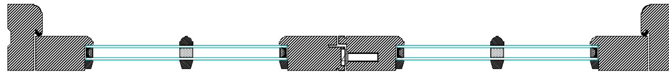
Glazed Panes with Applied Glazing Bars
