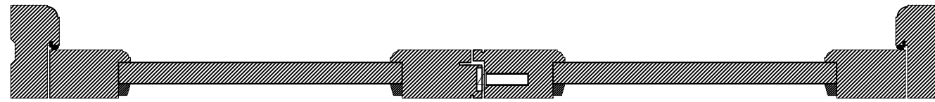
Timber Panels with Standard Beading
