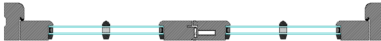
Glazed Panes with Applied Glazing Bars
